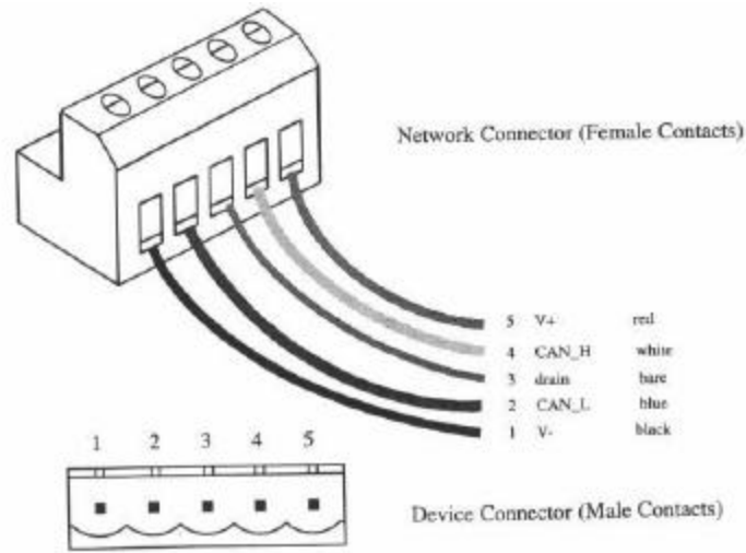
Figure 4-2 DeviceNet cable connector
